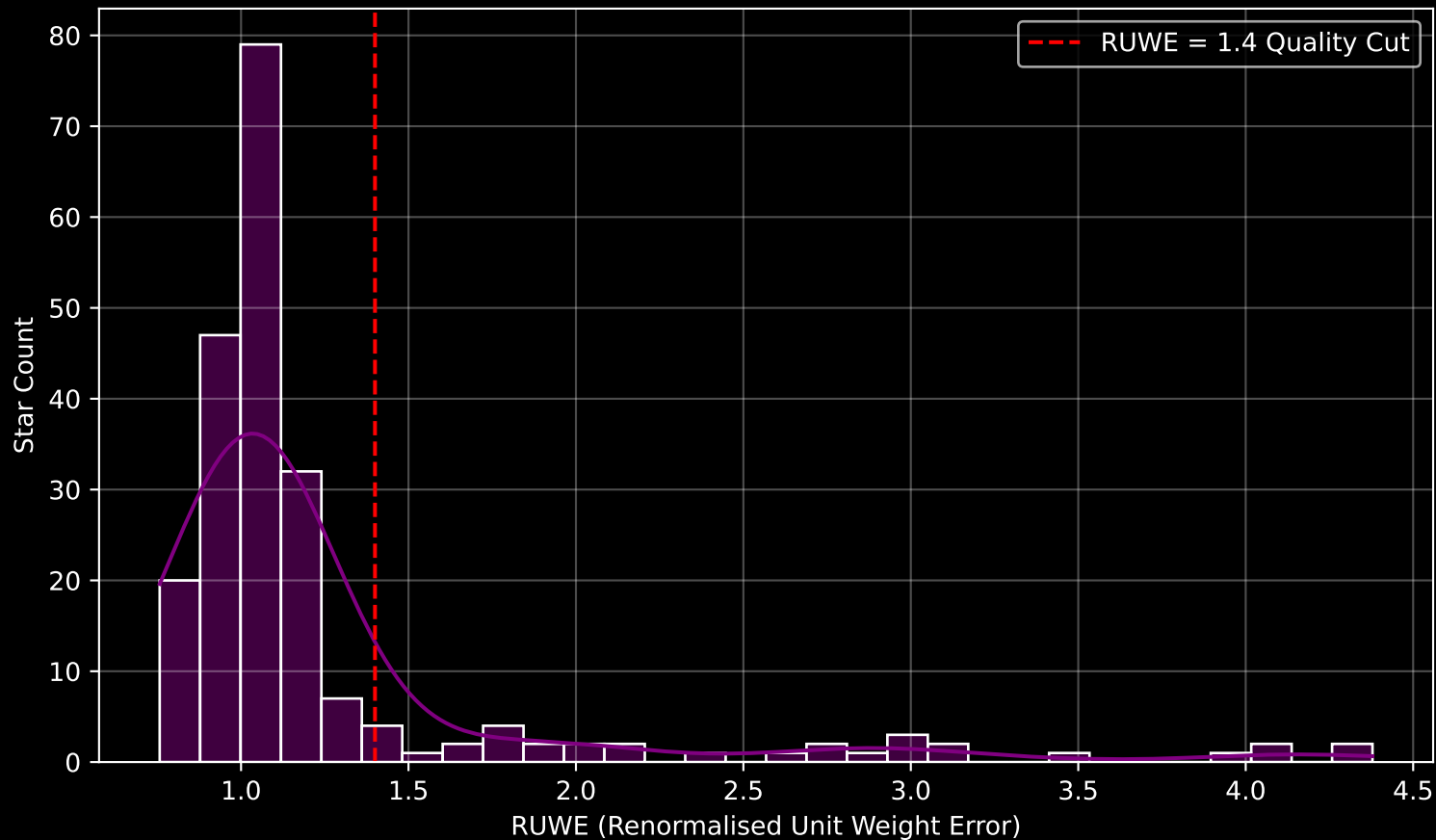
GALAH DR4 Field [7160] RUWE Distribution (n= 218)
