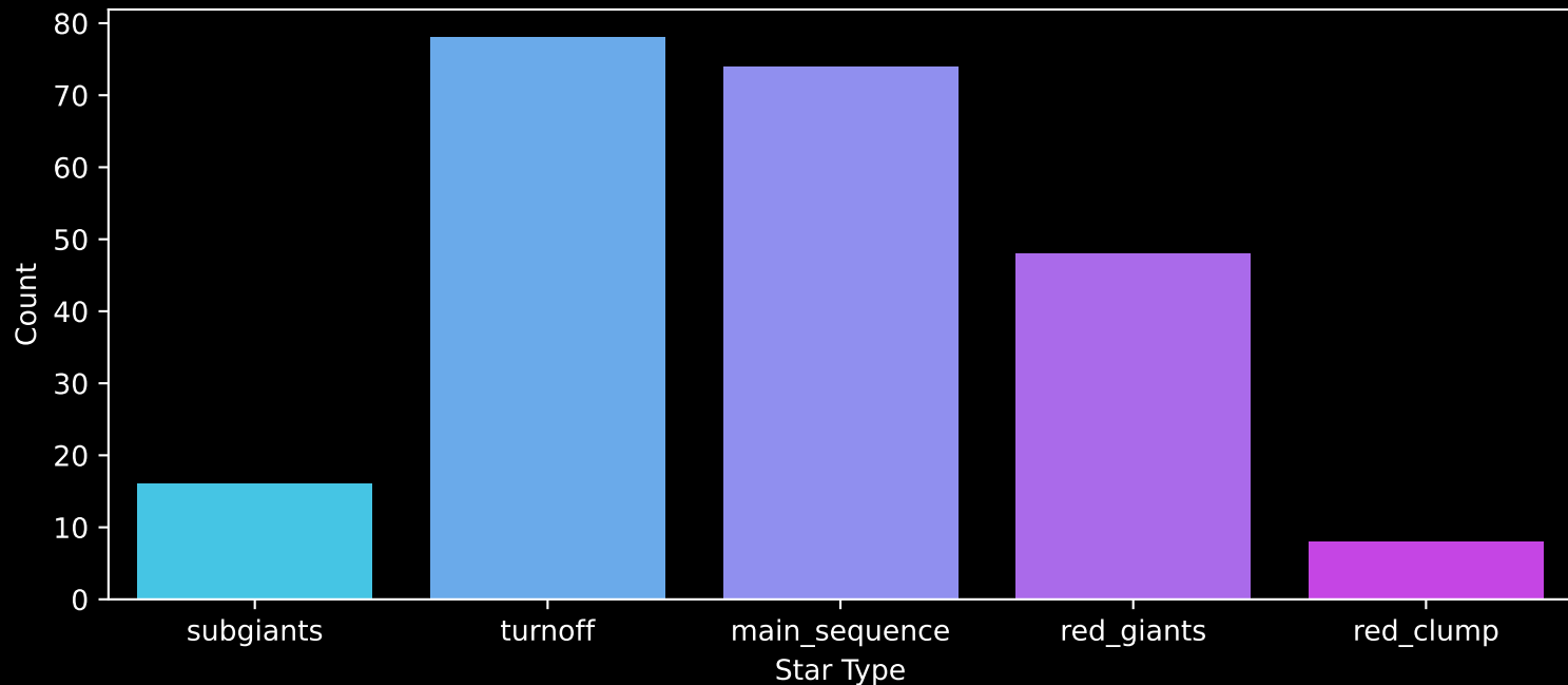
GALAH DR4 Field: [7160] Count plot of Star Type
