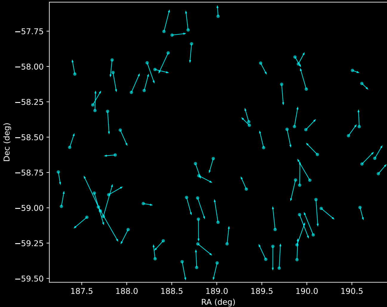
GALAH DR4 Noise Stream Proper Motion Vectors (n=77)
