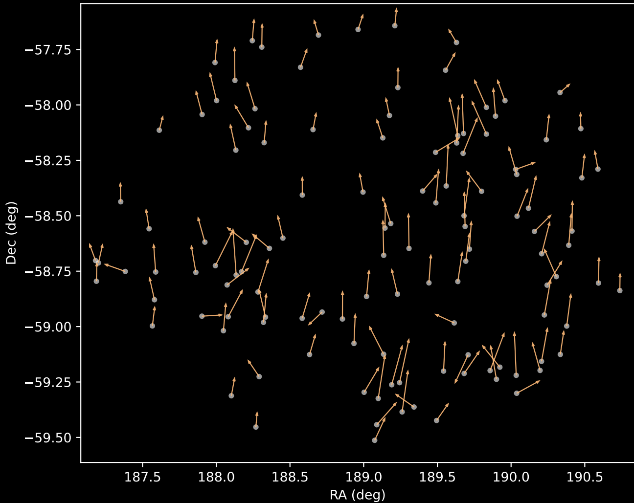
GALAH DR4 Cluster 3 Proper Motion Vectors (n=121)
