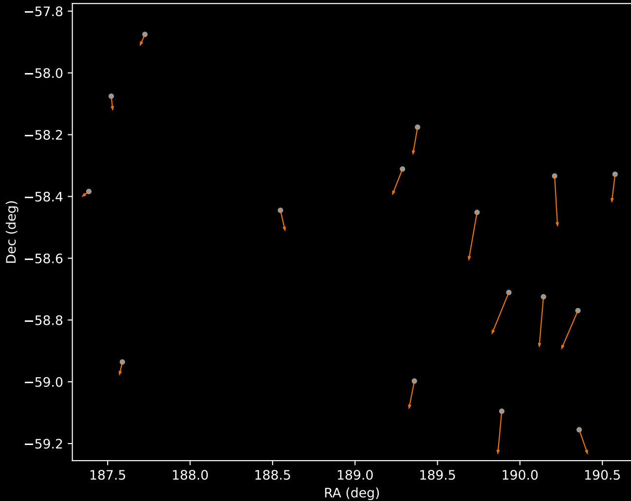
GALAH DR4 Cluster 2 Proper Motion Vectors (n=16)
